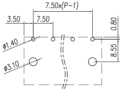
03-12P PCB LAYOUT
