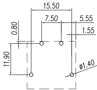
02P PCB LAYOUT
