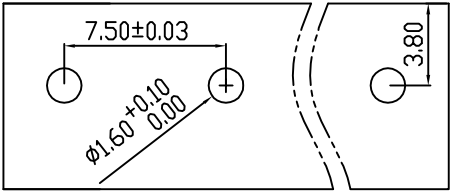
PCB LAYOUT
