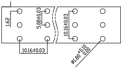
PCB Layout
