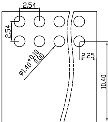
PCB Layout
