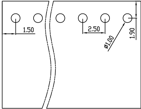
PCB Layout
